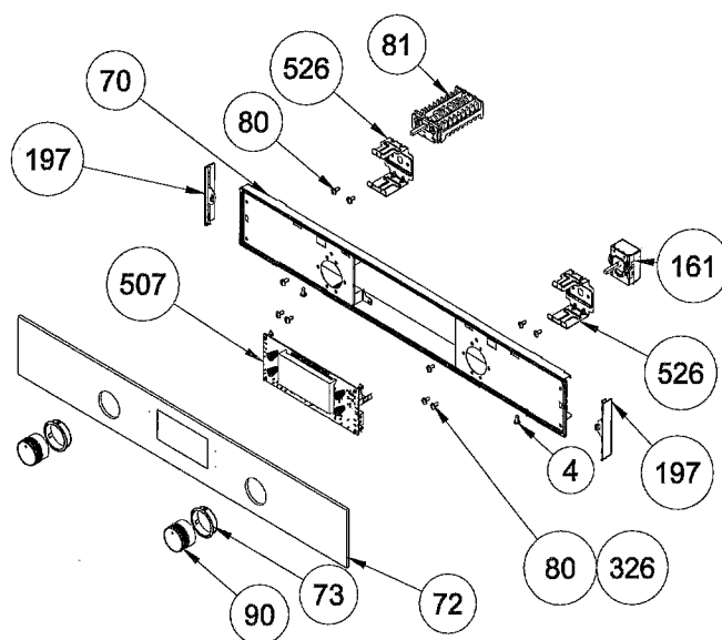
VISIO TOUCH GLASS CONTROL PANEL ASSEMBLY (OPTIONAL)
