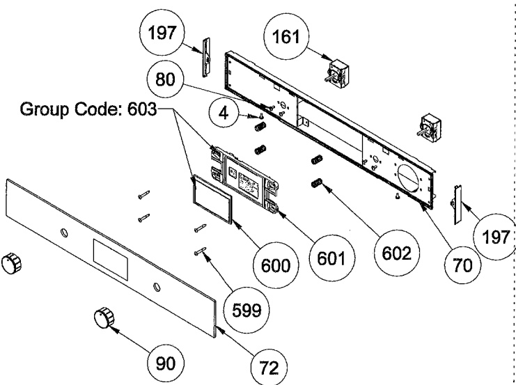
LCD SMART GLASS CONTROL PANEL ASSEMBLY (OPTIONAL)
