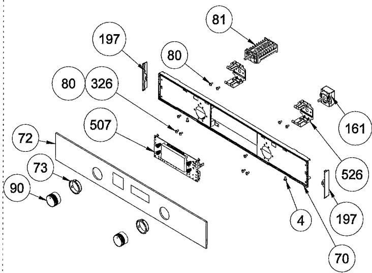
VISIO DISPLAY CONTROL PANEL ASSEMBLY (OPTIONAL)
