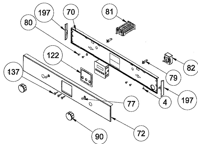
METAL CONTROL PANEL WITH DIGITAL TIMER ASSEMBLY (OPTIONAL)
